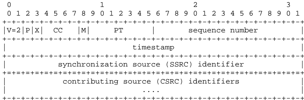
Figure 3. RTP header according to RFC 3550
